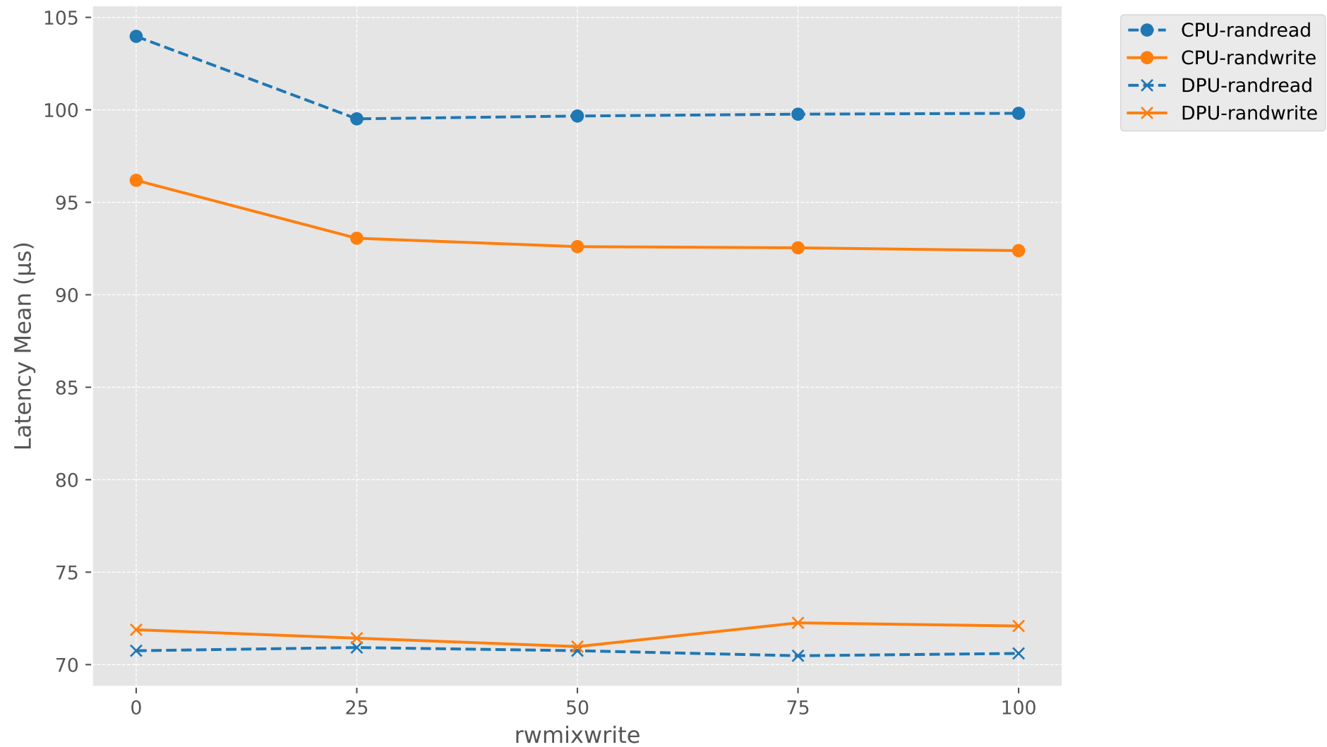
Latency Mean vs rwmixwrite
